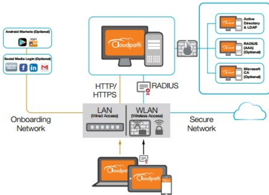
FIGURE 1 Cloudpath Security and Policy Management Platform
