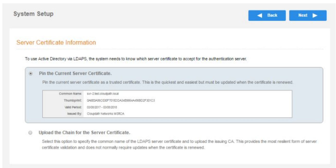
FIGURE 23 Authentication Server Certificate
