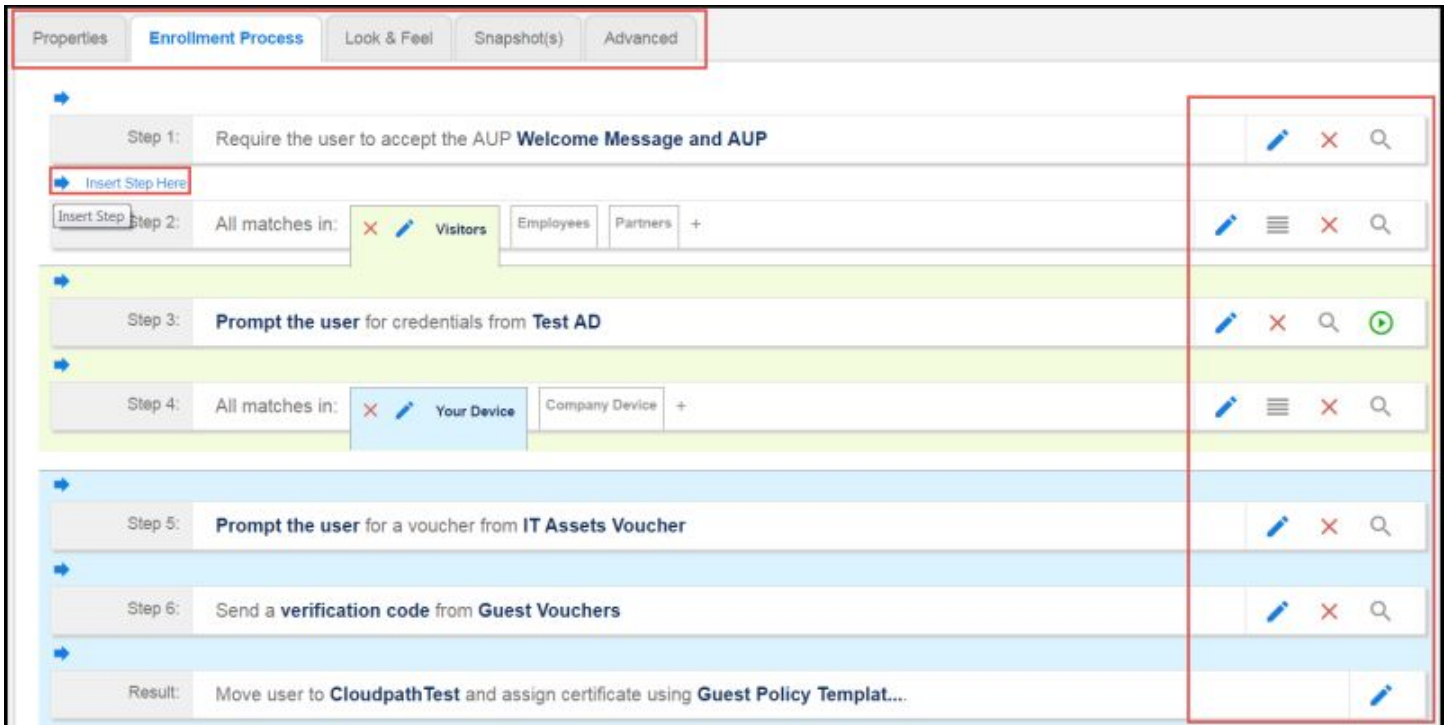
FIGURE 26 Workflow Configuration Page
