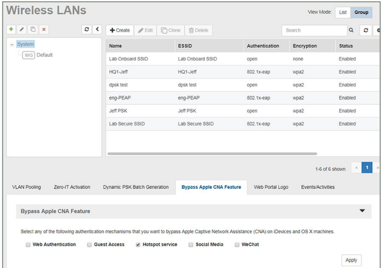
FIGURE 59 Enabling the Bypass Apple CNA Feature Globally on ZoneDirector
