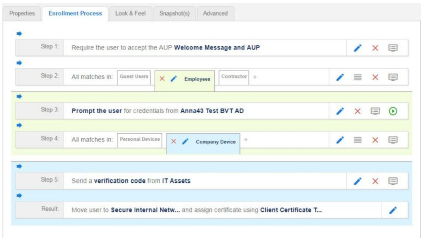
FIGURE 33 Workflow with Device Ownership Split
