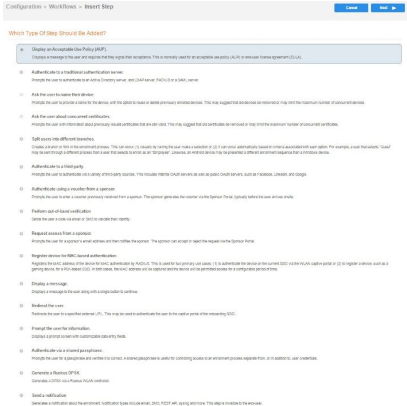
FIGURE 29 Enrollment Step Selection
